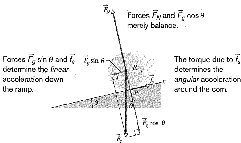
Fig. 11-8 A round uniform body of radius R rolls down a ramp. The forces that act on it are the gravitational force \vec{F}_g , a normal force \vec{F}_N , and a frictional force \vec{f}_s pointing up the ramp. (For clarity, vector \vec{F}_N has been shifted in the direction it points until its tail is at the center of the body.)
