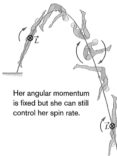
Fig. 11-17 The diver's angular momentum \vec{L} is constant throughout the dive, being represented by the tail \otimes of an arrow that is perpendicular to the plane of the figure. Note also that her center of mass (see the dots) follows a parabolic path.
