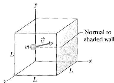
Fig. 19-4 A cubical box of edge length L , containing n moles of an ideal gas. A molecule of mass m and velocity \vec{v} is about to collide with the shaded wall of area L^2 . A normal to that wall is shown.
