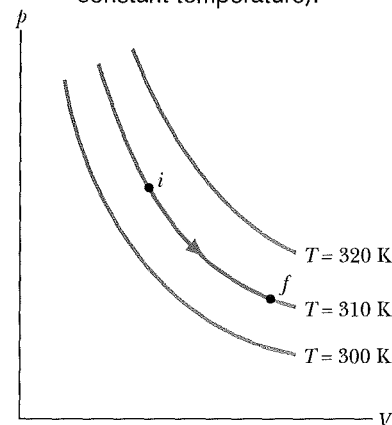
Fig. 19-2 Three isotherms on a p - V diagram. The path shown along the middle isotherm represents an isothermal expansion of a gas from an initial state i to a final state f . The path from f to i along the isotherm would represent the reverse process—that is, an isothermal compression.
