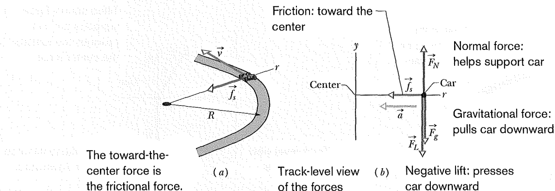
Fig. 6-10 (a) A race car moves around a flat curved track at constant speed v . The frictional force \vec{f}_s provides the necessary centripetal force along a radial axis r . (b) A free-body diagram (not to scale) for the car, in the vertical plane containing r .
