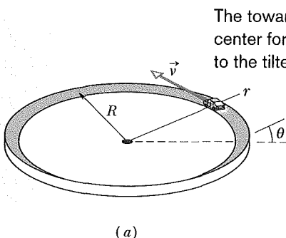
Fig. 6-11 (a) A car moves around a curved banked road at constant speed v . The bank angle is exaggerated for clarity. (b) A free-body diagram for the car, assuming that friction between tires and road is zero and that the car lacks negative lift. The radially inward component F_{Nr} of the normal force (along radial axis r ) provides the necessary centripetal force and radial acceleration.
