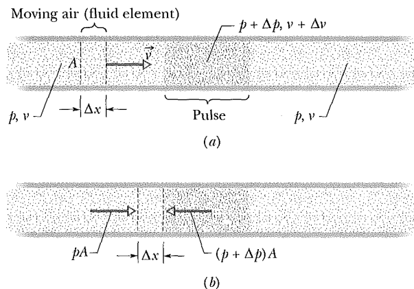
Fig. 17-3 A compression pulse is sent from right to left down a long air-filled tube. The reference frame of the figure is chosen so that the pulse is at rest and the air moves from left to right. (a) An element of air of width \Delta x moves toward the pulse with speed v . (b) The leading face of the element enters the pulse. The forces acting on the leading and trailing faces (due to air pressure) are shown.
