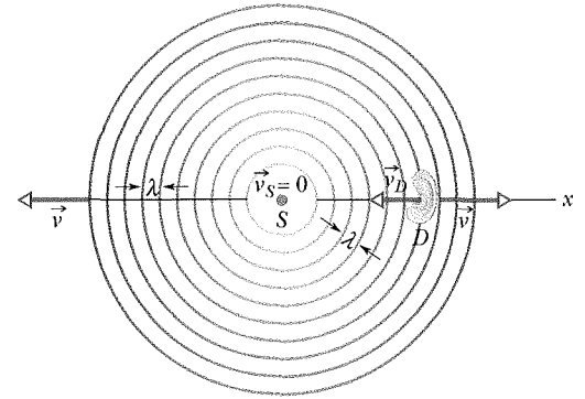
Fig. 17-18 A stationary source of sound S emits spherical wavefronts, shown one wavelength apart, that expand outward at speed v . A sound detector D , represented by an ear, moves with velocity \vec{v}_D toward the source. The detector senses a higher frequency because of its motion.
