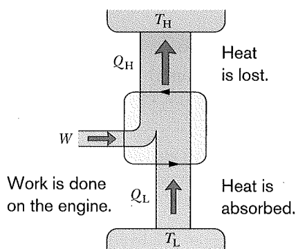
Fig. 20-14 The elements of a refrigerator. The two black arrowheads on the central loop suggest the working substance operating in a cycle, as if on a p - V plot. Energy is transferred as heat Q_L to the working substance from the low-temperature reservoir. Energy is transferred as heat Q_H to the high-temperature reservoir from the working substance. Work W is done on the refrigerator (on the working substance) by something in the environment.
