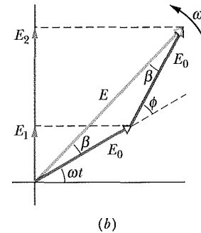
Fig. 35-13 (a) Phasors representing, at time t , the electric field components given by Eqs. 35-20 and 35-21. Both phasors have magnitude E_0 and rotate with angular speed \omega . Their phase difference is \phi . (b) Vector addition of the two phasors gives the phasor representing the resultant wave, with amplitude E and phase constant \beta .
