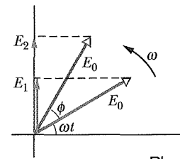
(a) Phasors that represent waves can be added to find the net wave.
