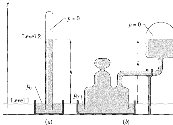
Fig. 14-5 (a) A mercury barometer. (b) Another mercury barometer. The distance h is the same in both cases.
