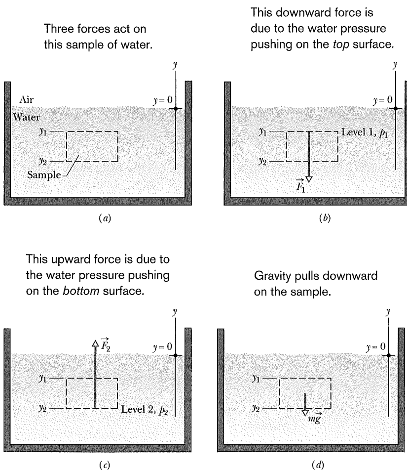
Fig. 14-2 (a) A tank of water in which a sample of water is contained in an imaginary cylinder of horizontal base area A . (b)–(d) Force \vec{F}_1 acts at the top surface of the cylinder; force \vec{F}_2 acts at the bottom surface of the cylinder; the gravitational force on the water in the cylinder is represented by m\vec{g} . (e) A free-body diagram of the water sample.
