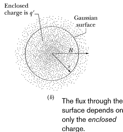
Fig. 23-19 The dots represent a spherically symmetric distribution of charge of radius R , whose volume charge density \rho is a function only of distance from the center. The charged object is not a conductor, and therefore the charge is assumed to be fixed in position. A concentric spherical Gaussian surface with r > R is shown in (a). A similar Gaussian surface with r < R is shown in (b).
