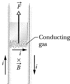
Fig. 29-10 (a) A rail gun, as a current i is set up in it. The current rapidly causes the conducting fuse to vaporize. (b) The current produces a magnetic field \vec{B} between the rails, and the field causes a force \vec{F} to act on the conducting gas, which is part of the current path. The gas propels the projectile along the rails, launching it.
