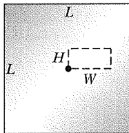
Fig. 32-28 Problem 6.
