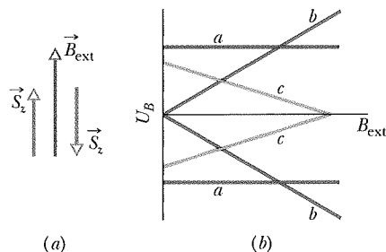
Fig. 32-22 Question 4.
