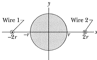
Fig. 32-27 Problem 4.
