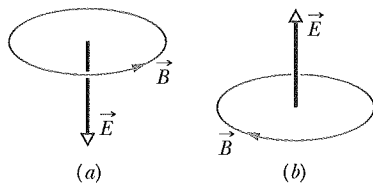
Fig. 32-21 Question 3.
