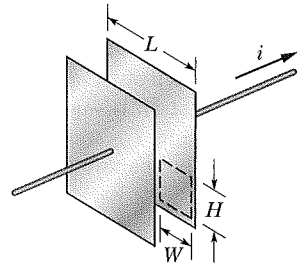
Fig. 32-41 Problem 67.
