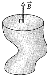
Fig. 32-26 Problem 2.
