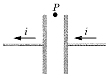
Fig. 32-20 Question 2.
