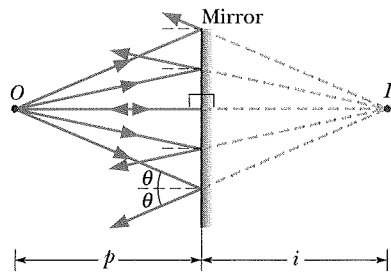
Fig. 34-2 A point source of light O , called the object , is at a perpendicular distance p in front of a plane mirror. Light rays reaching the mirror from O reflect from the mirror. If your eye intercepts some of the reflected rays, you perceive a point source of light I to be behind the mirror, at a perpendicular distance i . The perceived source I is a virtual image of object O .
