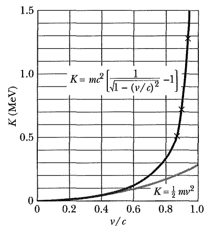
Fig. 37-13 The relativistic (Eq. 37-52) and classical (Eq. 37-51) equations for the kinetic energy of an electron, plotted as a function of v/c , where v is the speed of the electron and c is the speed of light. Note that the two curves blend together at low speeds and diverge widely at high speeds. Experimental data (at the \times marks) show that at high speeds the relativistic curve agrees with experiment but the classical curve does not.
