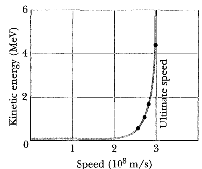
Fig. 37-2 The dots show measured values of the kinetic energy of an electron plotted against its measured speed. No matter how much energy is given to an electron (or to any other particle having mass), its speed can never equal or exceed the ultimate limiting speed c . (The plotted curve through the dots shows the predictions of Einstein's special theory of relativity.)
