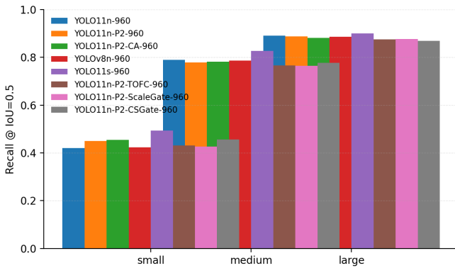
Fig. 3. Scale-wise recall on the VisDrone2019-DET validation set. The figure is generated from audited scale-group CSV files.
