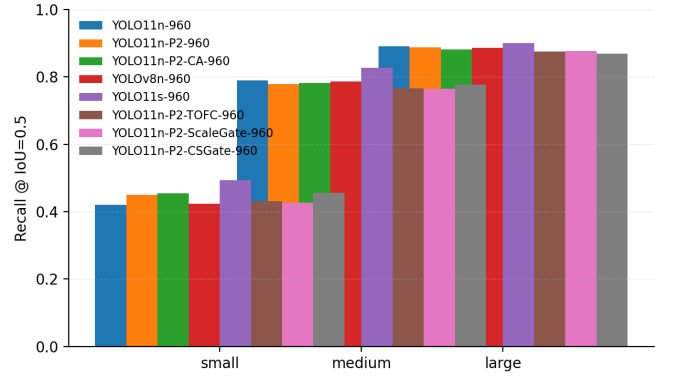
Fig. 2. Scale-wise recall on the VisDrone2019-DET validation set. The figure is generated from audited scale-group CSV files.
