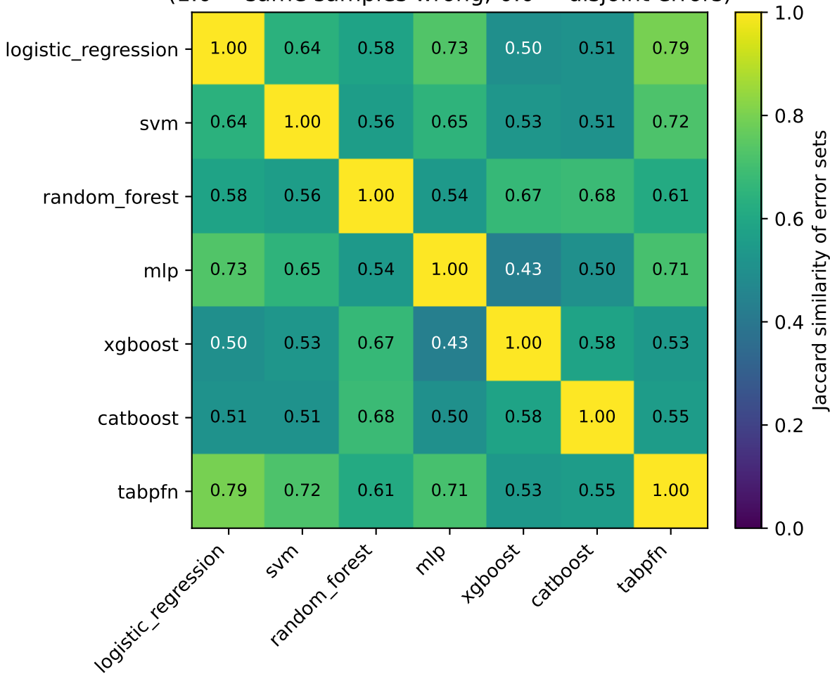
liver — pairwise Jaccard of OOF error sets (1.0 = same samples wrong; 0.0 = disjoint errors)
