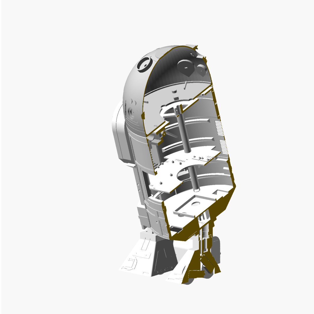
cad/section.png - the native OpenSCAD model cut on the centre plane. Battery bay, electronics deck, ring seam and the dome bearing seat.
