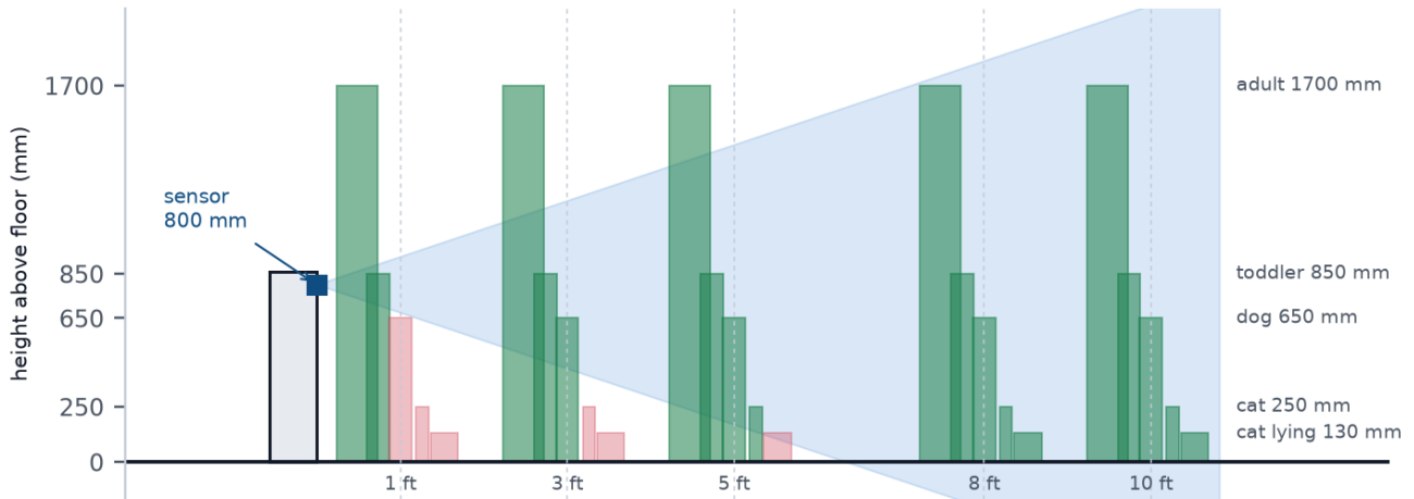
sensor at 800 mm, 45 deg vertical field of view, 0 deg down-tilt (green = inside the beam, red = missed)
