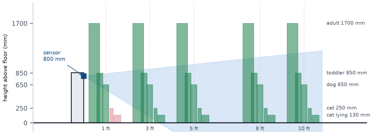
sensor at 800 mm, 45 deg vertical field of view, 15 deg down-tilt (green = inside the beam, red = missed)
