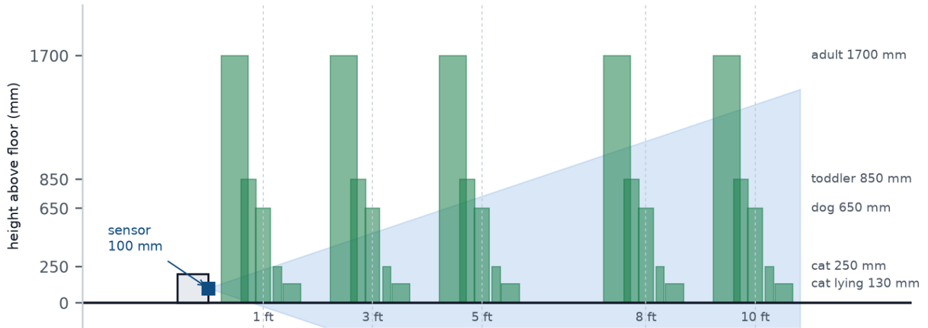
VL53L5CX at 100 mm, 45 deg vertical, no tilt (green = inside the beam, red = missed)
