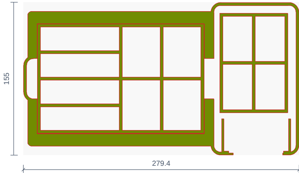
PLAN SECTION / Z = 127
