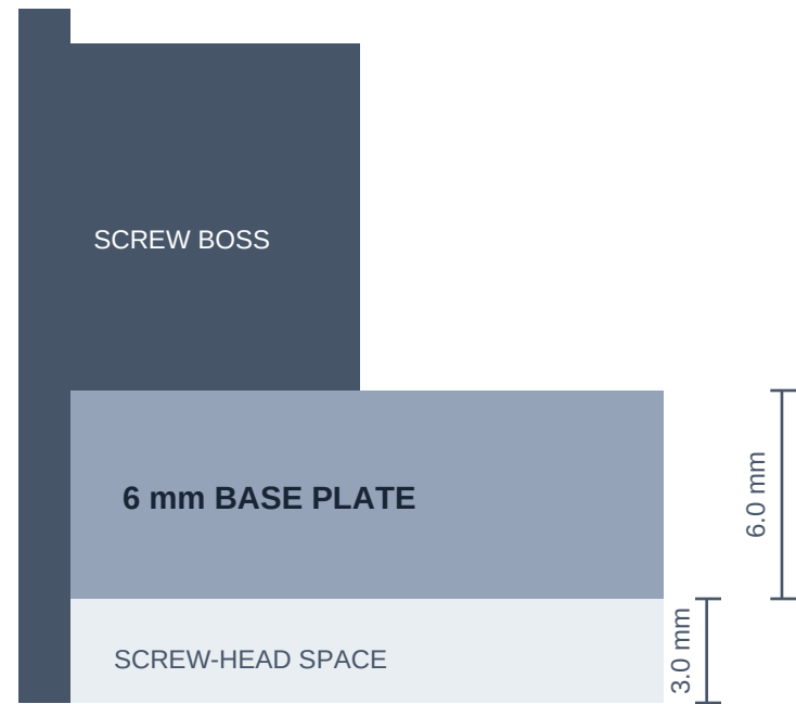
BODY BOTTOM / Z = 0
