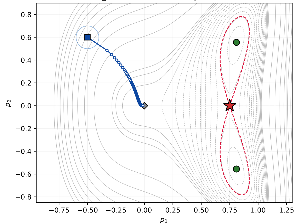
(c) R-DFO, \zeta = 10.0 first_order in 4 iters, limit saddle at 9.6\text{e-}16
