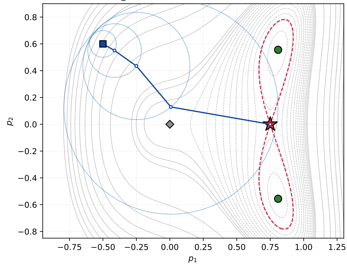
(c) R-DFO, \zeta = 10.0 first_order in 4 iters, limit saddle at 9.6\text{e-}16
