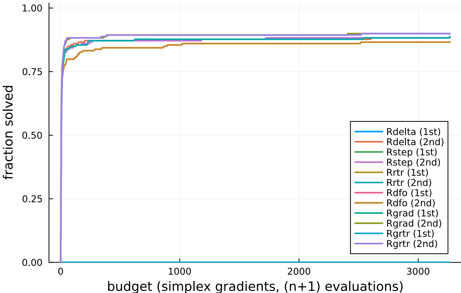
P3: data profile, objective evaluations
