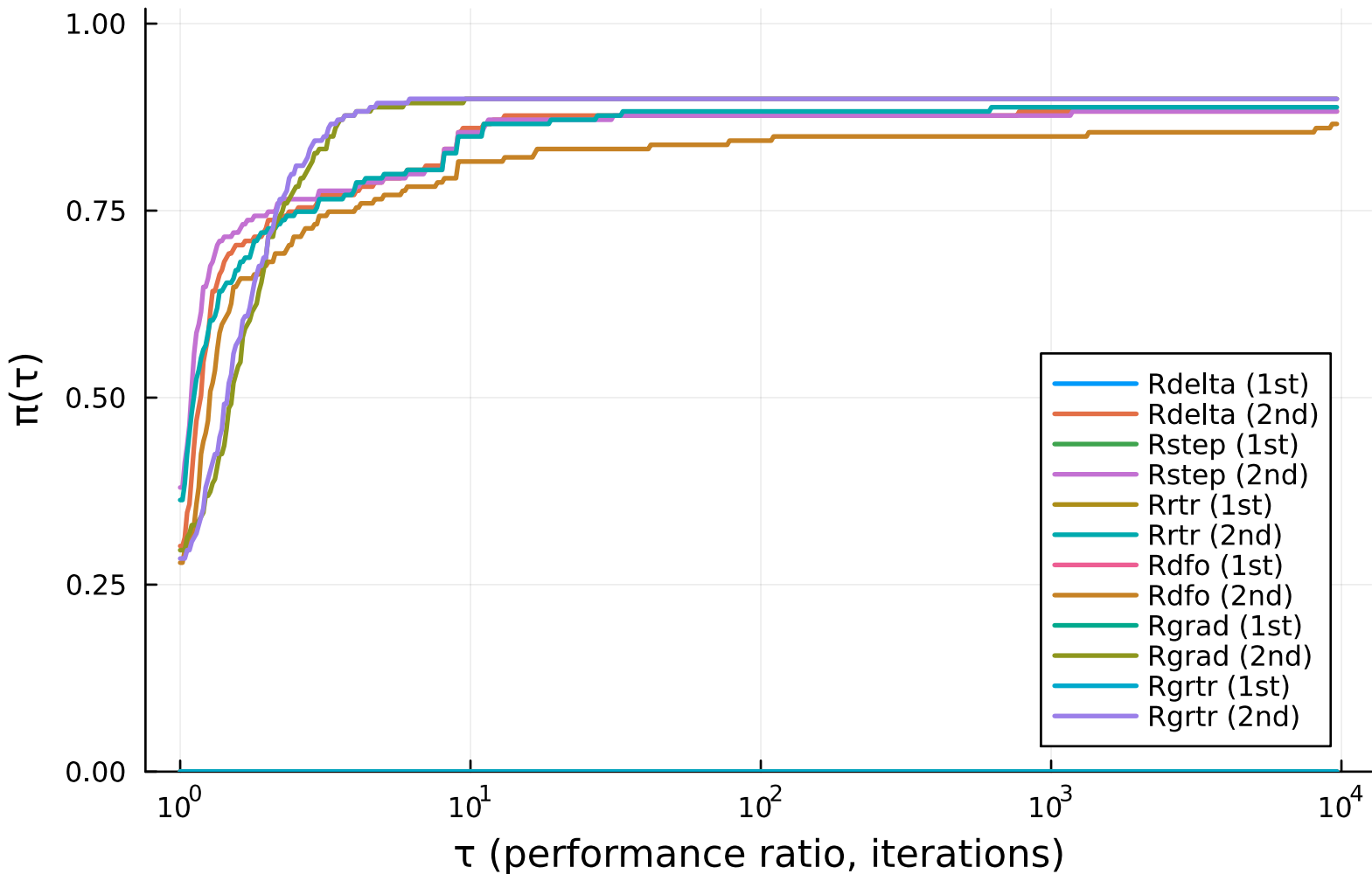
P3: both arms, second-order criterion, n \leq 200
