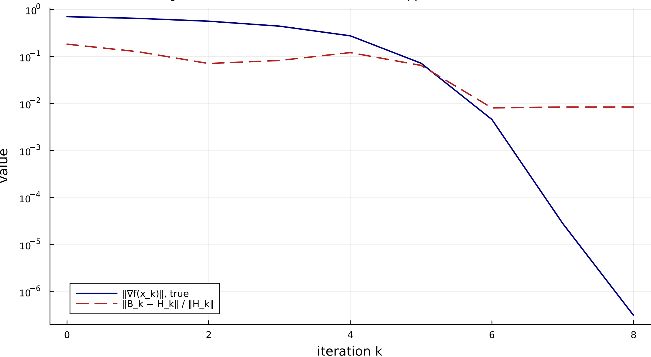
Figure 1. The BHHH error falls as the run approaches the solution
