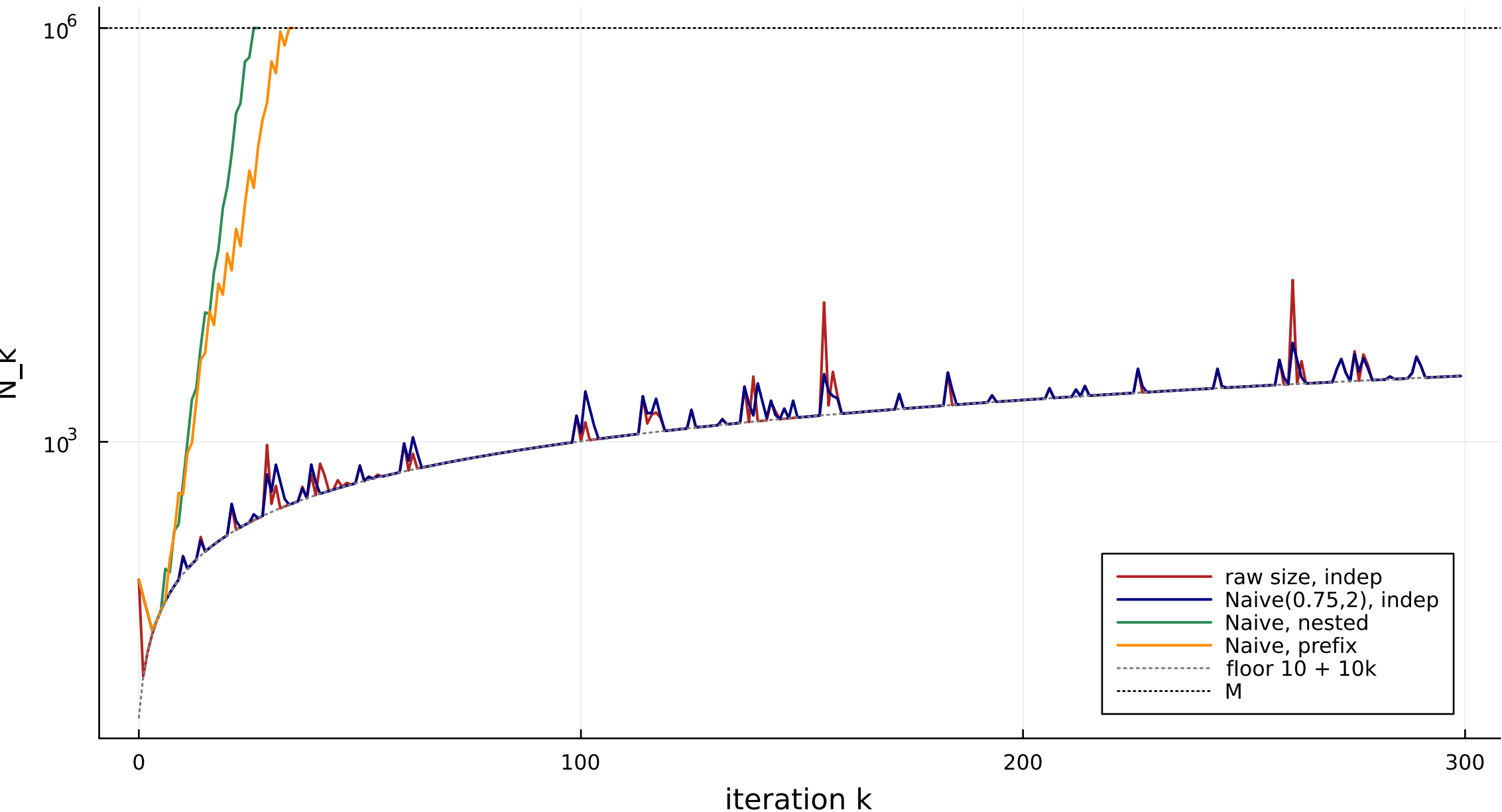
Figure 2. The sample size under the four sampled arms
