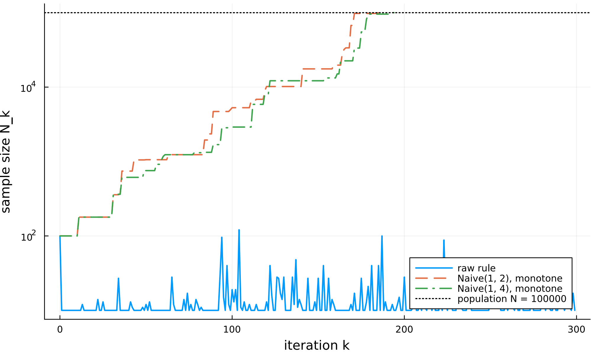
Sample size, raw rule against Naive(1,b) smoothing
