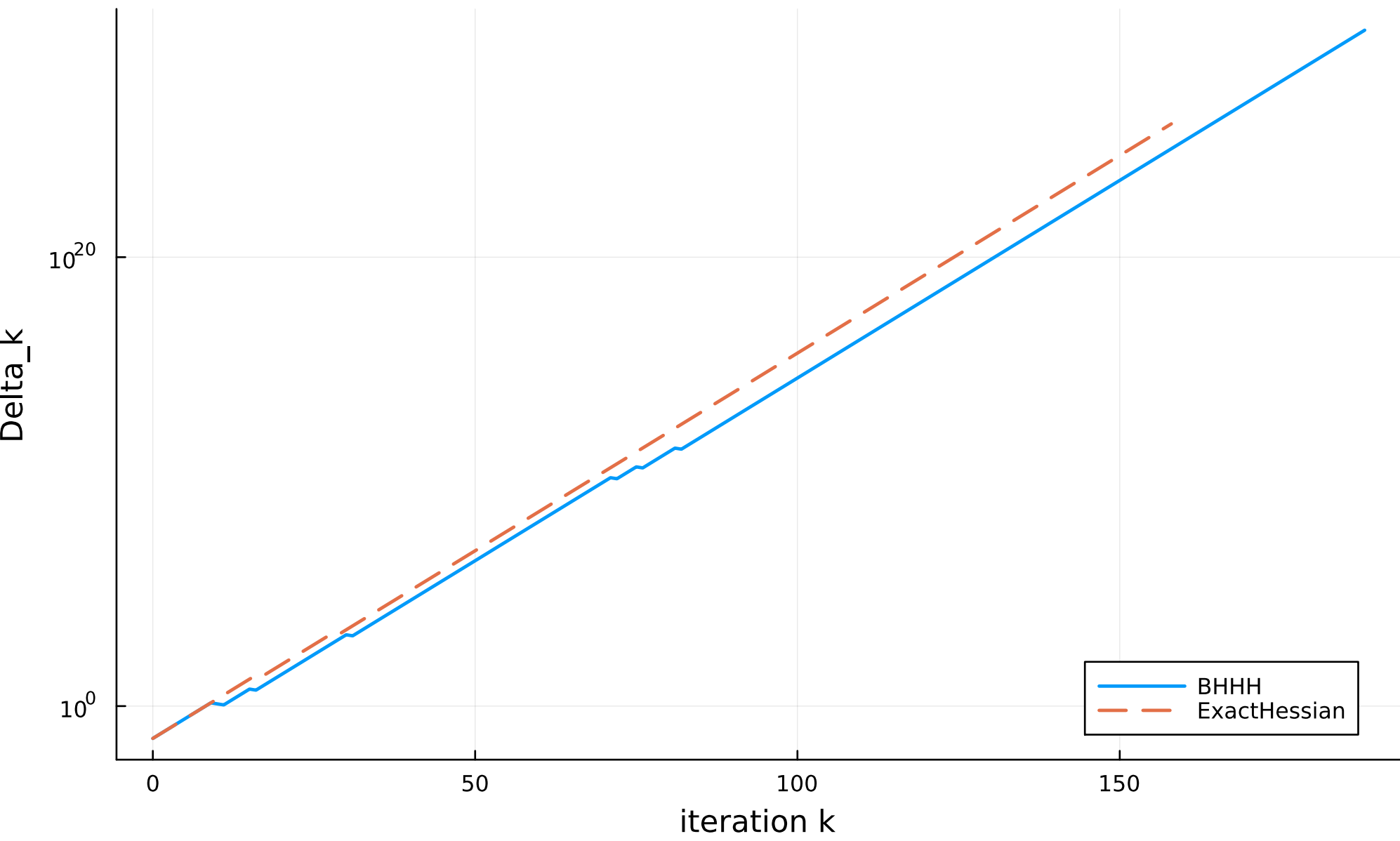
Trust-region radius under two model Hessians
