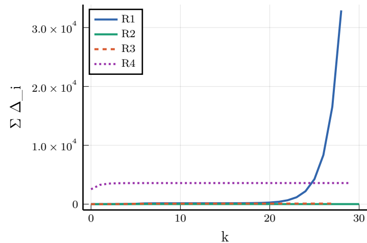
CUBE
