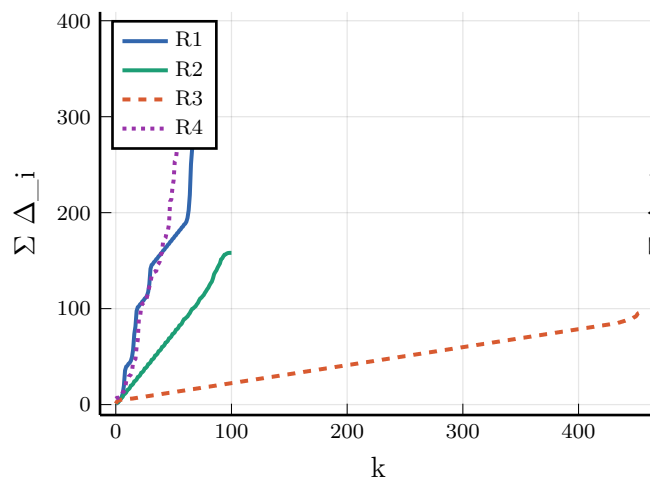
SNAIL
