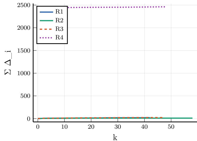
CUBE
