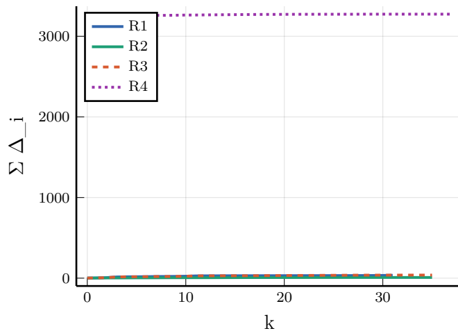
SNAIL
