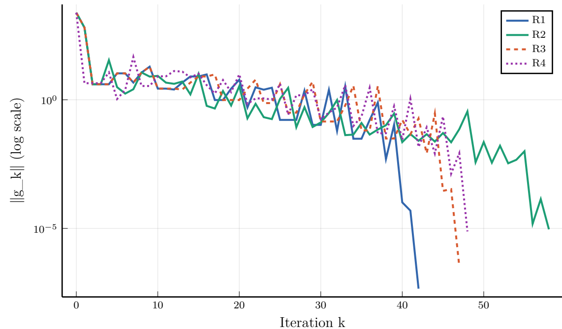
Gradient norm \|g_k\| — CUBE
