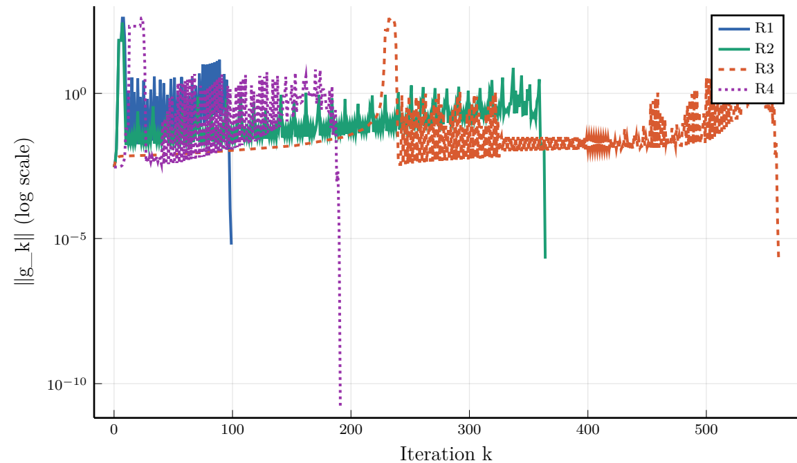
Gradient norm \|g_k\| — ROSENBRTU
