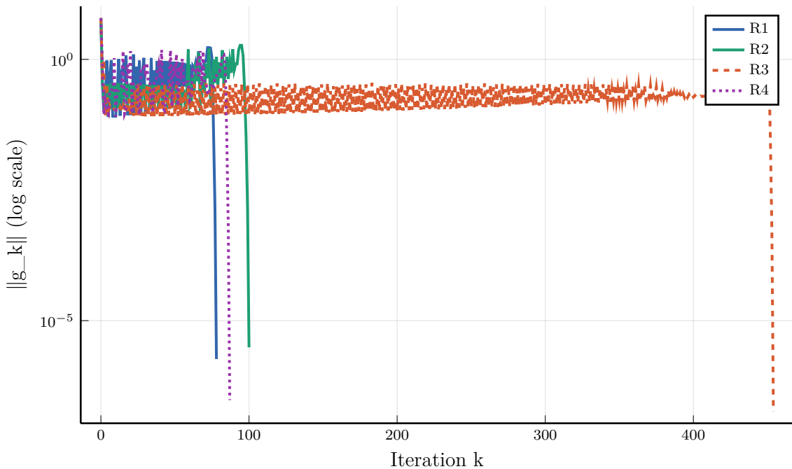
Gradient norm \|g_k\| — SNAIL
