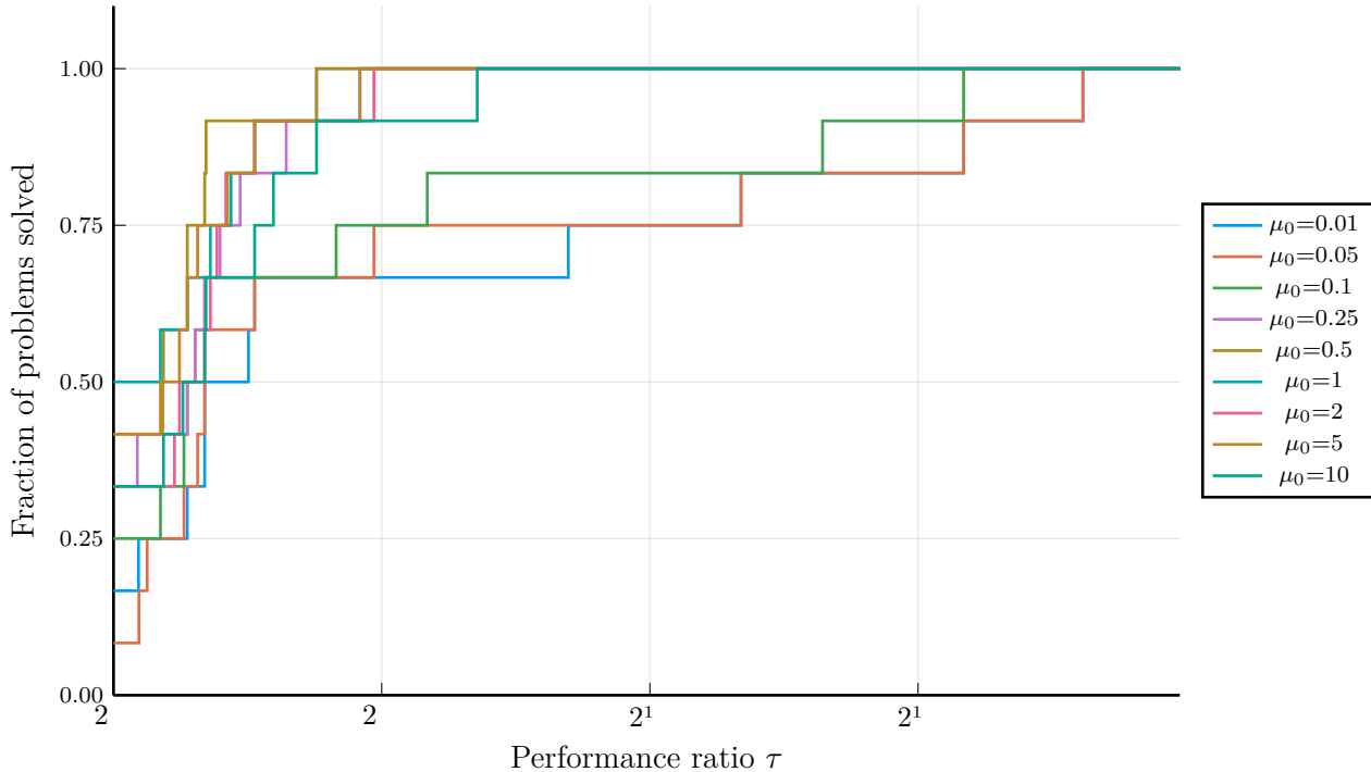
R4 performance profile — varying \mu_0
