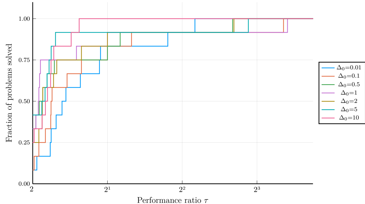
R3: performance profile — varying \Delta_0
