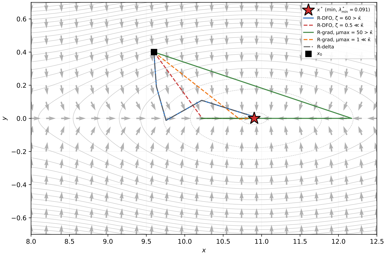
Trajectories on f(x, y) = \sin(x)/x + y^2 near x^* \approx (10.90, 0)
