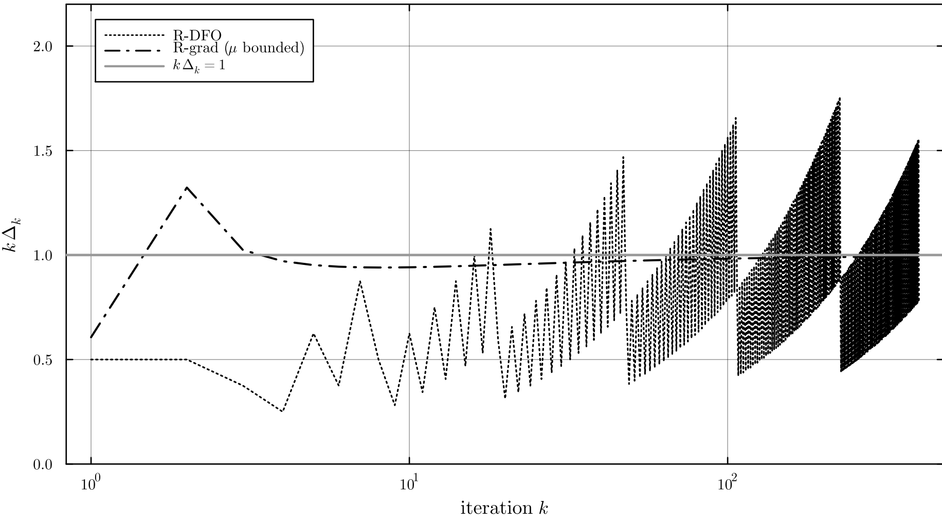
Fig. 5: k\Delta_k \rightarrow 1 for R-grad; \Theta(1/k) band for R-DFO
