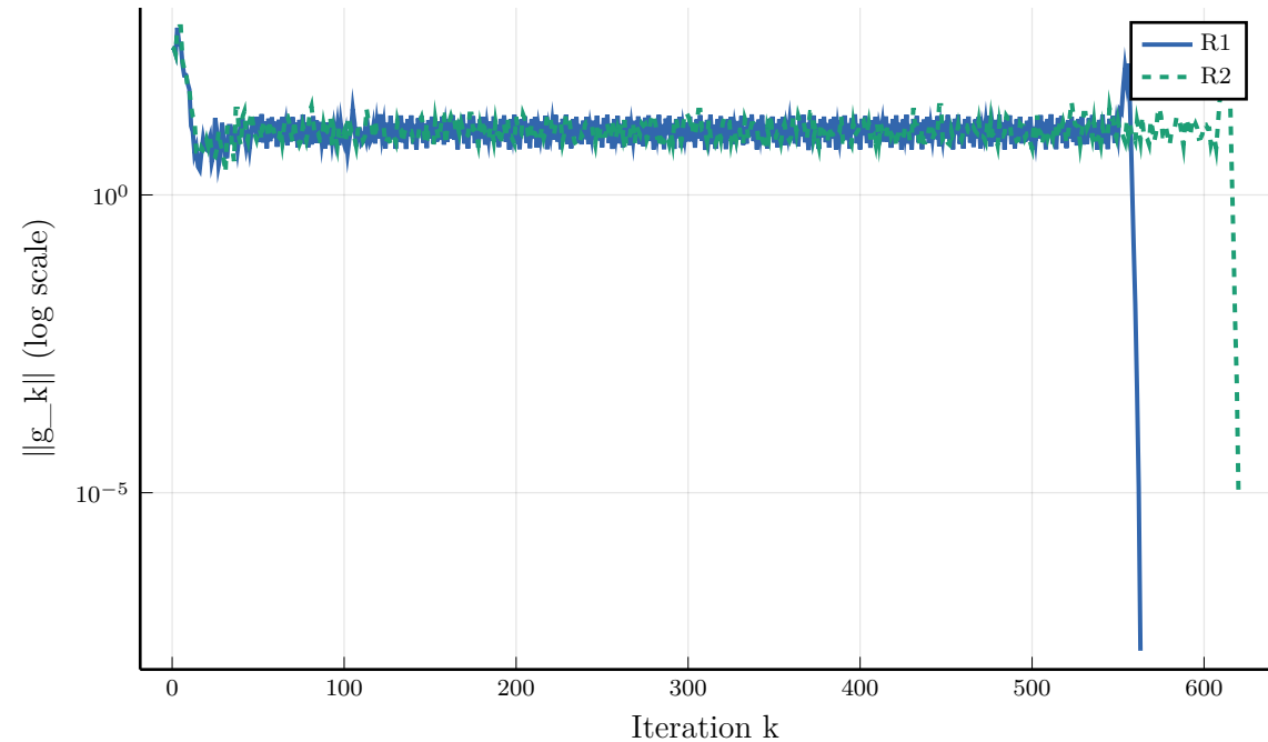
Gradient norm \|g_k\| — GENROSEB
