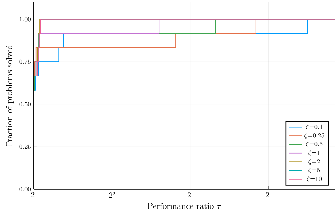
R3 performance profile — varying \zeta
