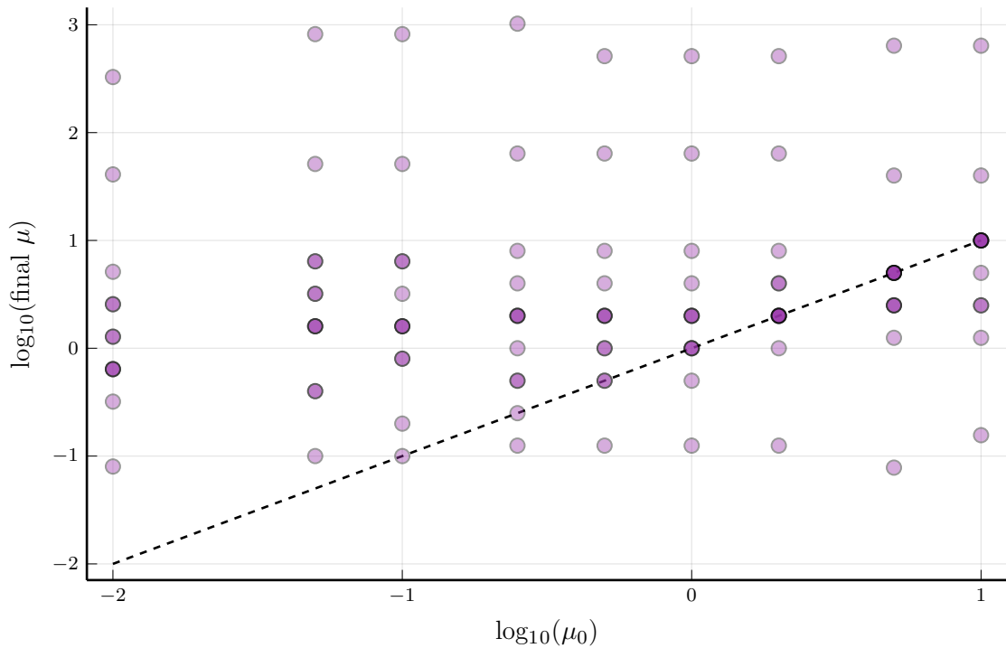
R4: \mu drift
