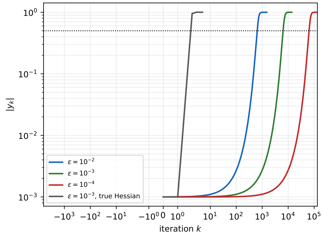
(a) escape along the unstable direction
