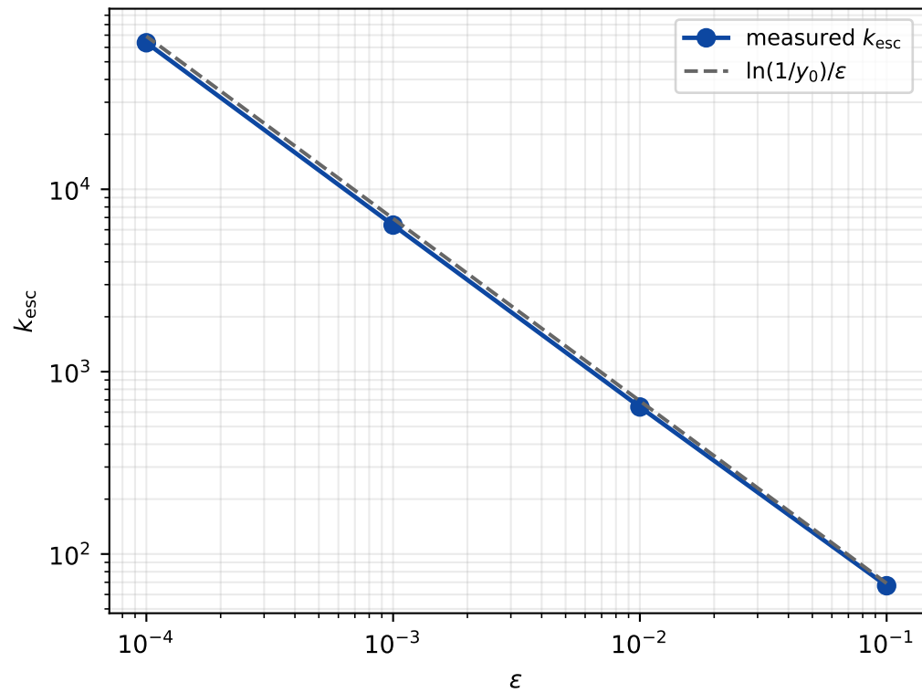
(b) escape time scales as 1/\epsilon
