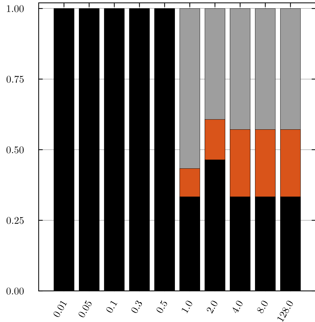
LBFGS
