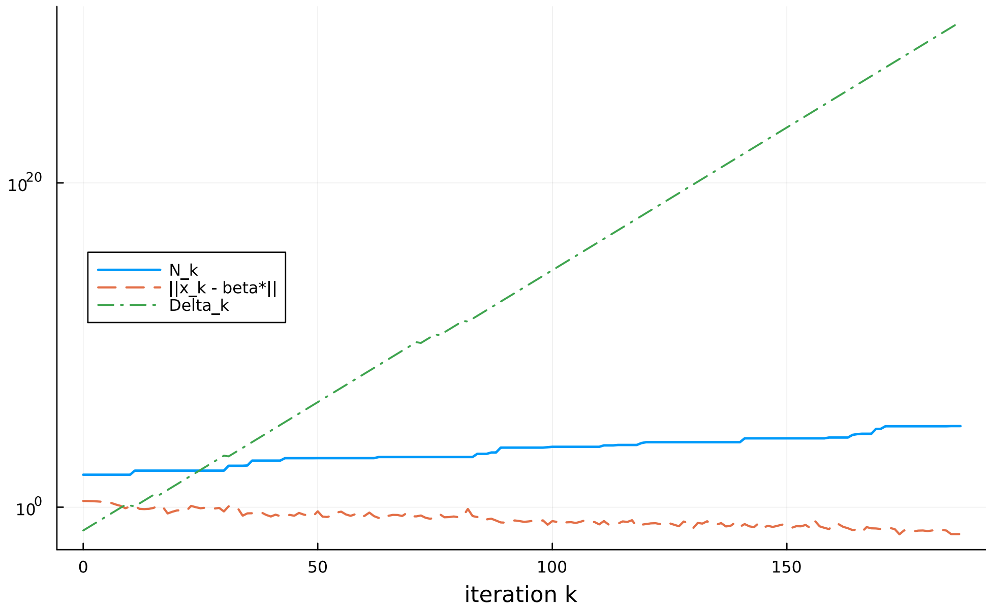
Sample size and distance to \beta^* , Naive(1,2)
