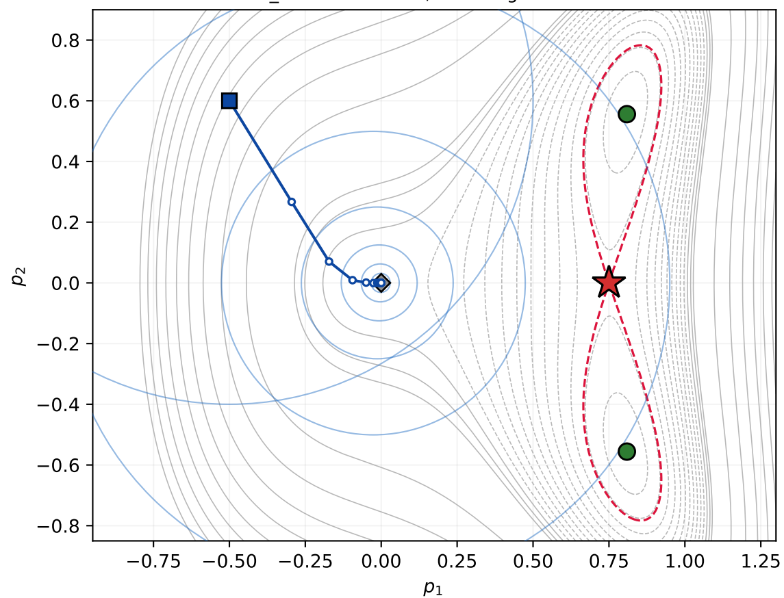
(d) R-DFO, \zeta = 20 first_order in 16 iters, limit origin at 1.3\text{e-}05
