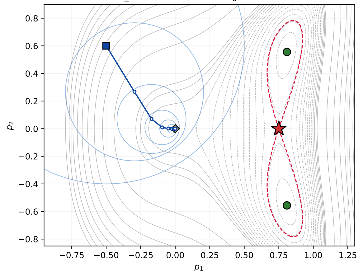
(c) R-DFO, \zeta = 0.1 first_order in 16 iters, limit origin at 1.3\text{e-}05
