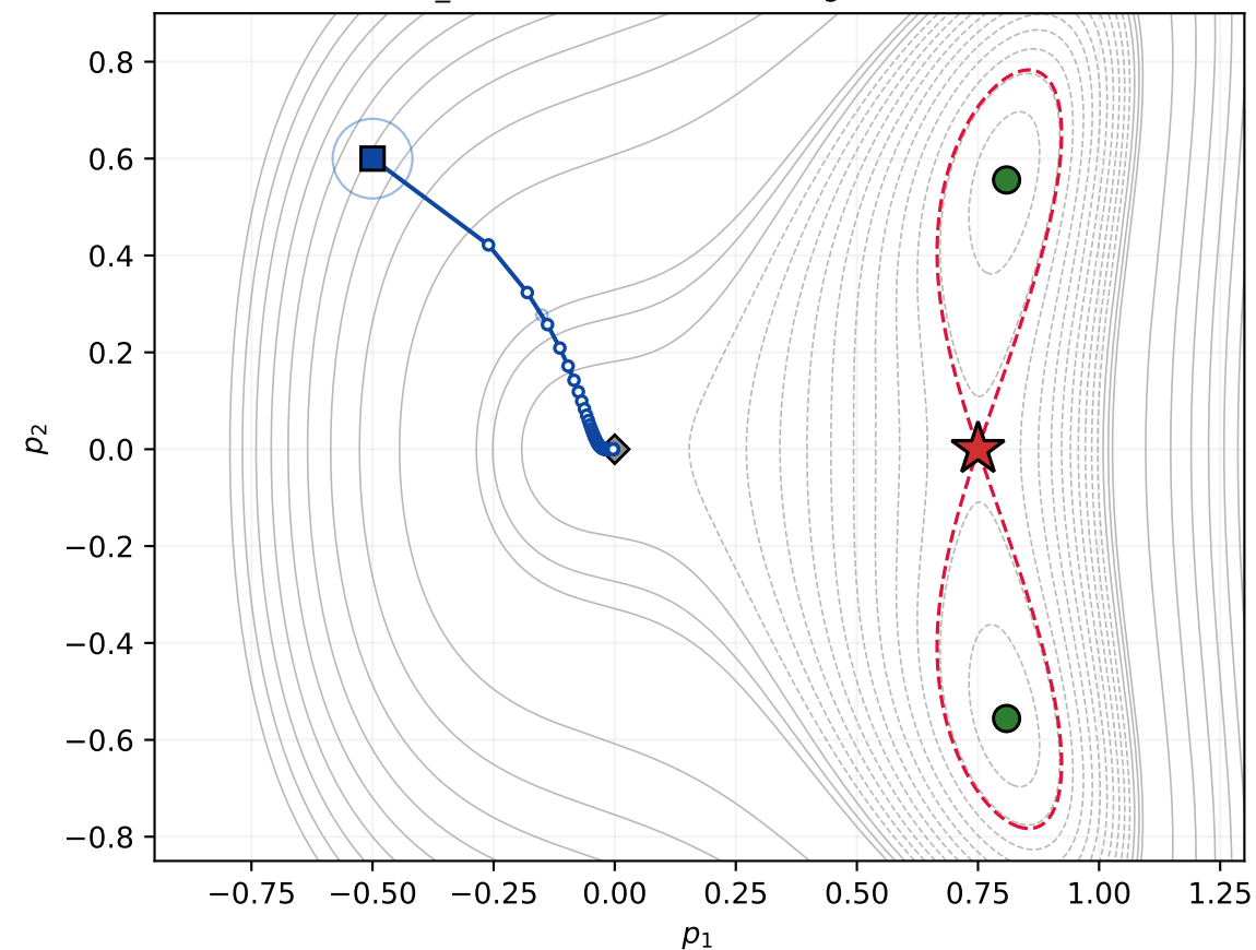
(c) R-DFO, \zeta = 0.1 first_order in 16 iters, limit origin at 1.3\text{e-}05
