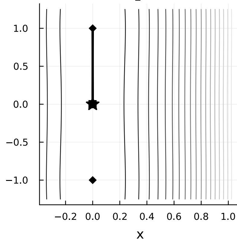
x_0 = 0.8 , \text{eps} = 0.01 stalled, k_{\text{esc}} = 639
