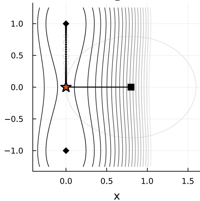
x_0 = 0.8 , \text{eps} = 0.1 stalled, k_{\text{esc}} = 67
