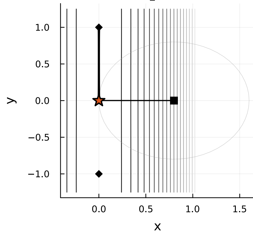
x_0 = 0.8 , \text{eps} = 0.001 stalled, k_{\text{esc}} = 6362
