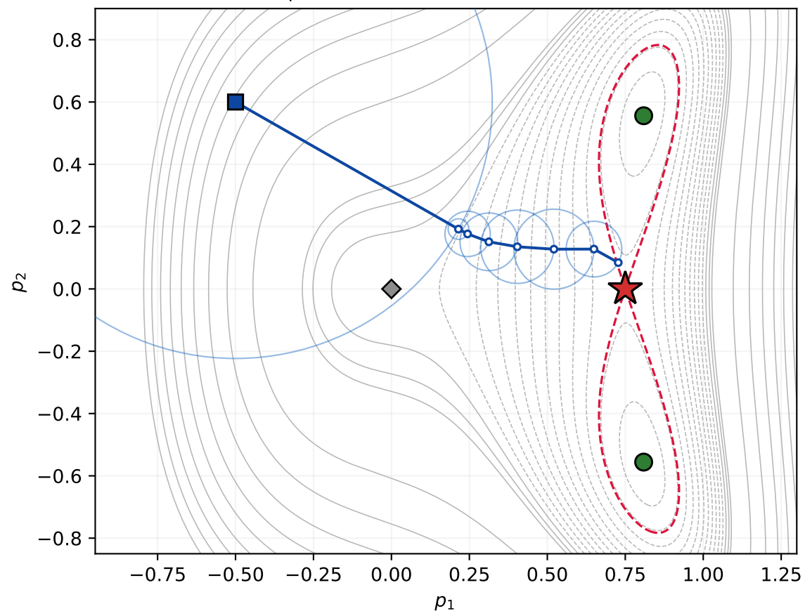
(d) R-grad capped, \mu_{\max} = 0.05 first_order in 5 iters, limit saddle at 6.9\text{e-}17
