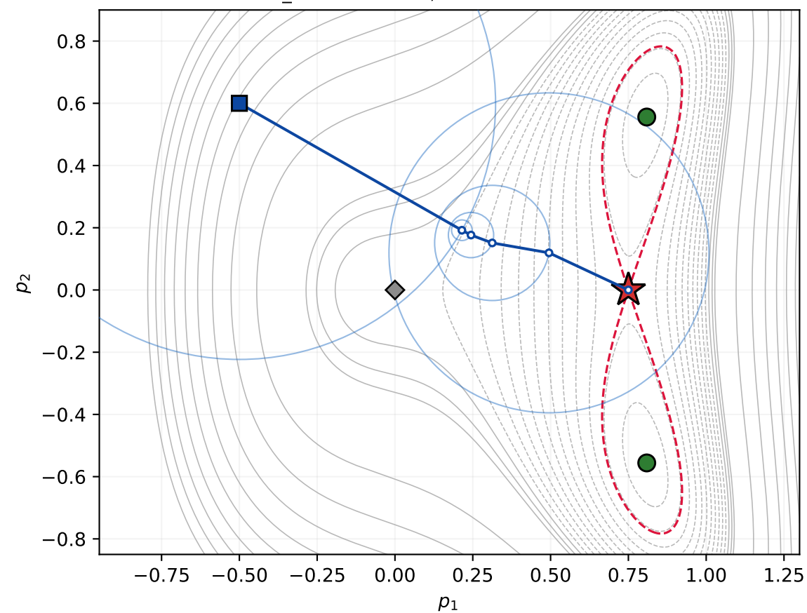
(c) R-grad capped, \mu_{\max} = 0.05 first_order in 5 iters, limit saddle at 6.9\text{e-}17
