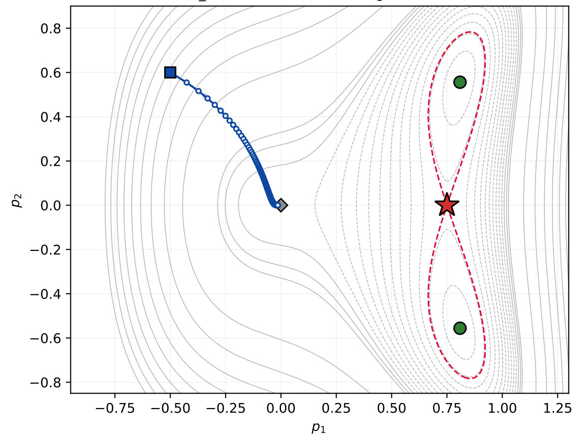
(c) R-grad capped, \mu_{\max} = 0.05 first_order in 5 iters, limit saddle at 6.9\text{e-}17
