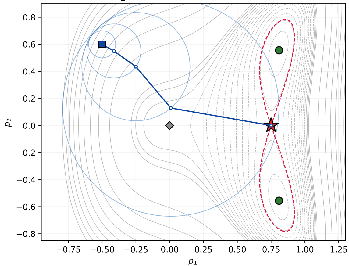
(d) R-DFO, \zeta = 0.1 first_order in 4 iters, limit saddle at 9.6\text{e-}16
