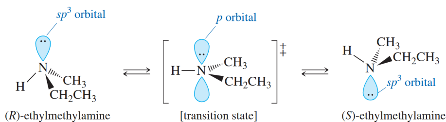
Figure 19.1 Nitrogen Inversion
