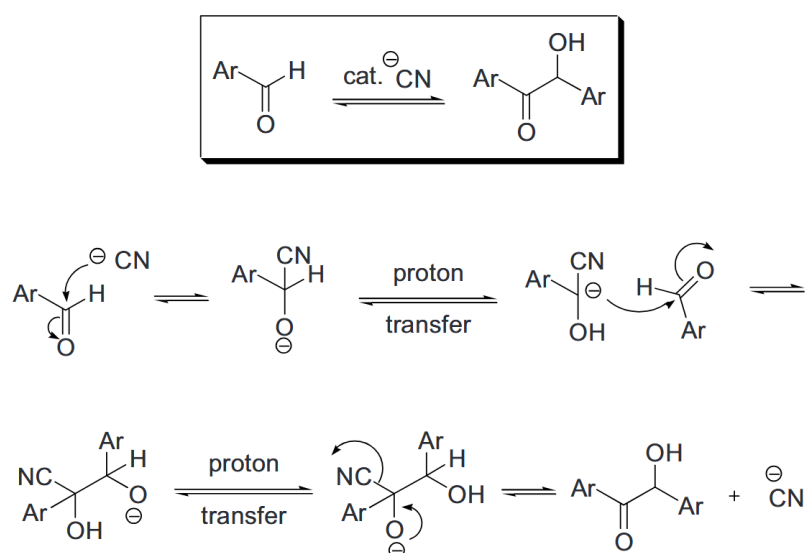
Figure 18.1 Benzoin Condensation
