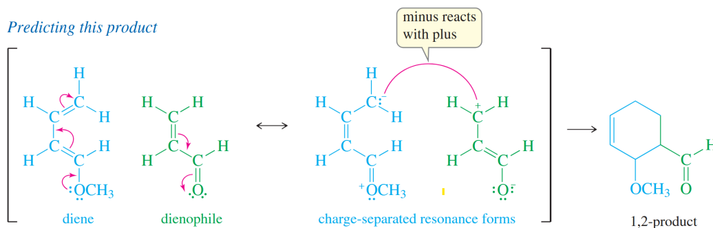
Figure 15.8 Formation of 1,2-product
