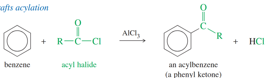
Figure 17.7 Friedel–Crafts acylation
