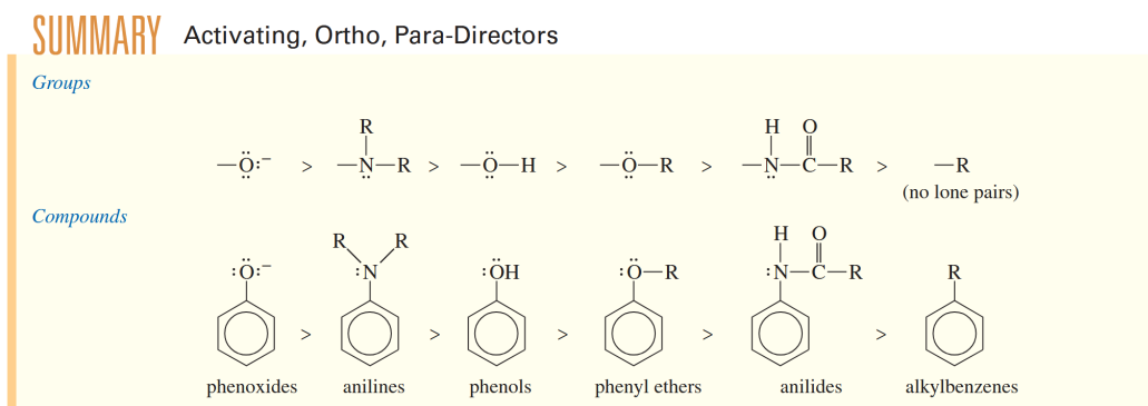
Figure 17.2 Activating, Ortho, Para-Directors
