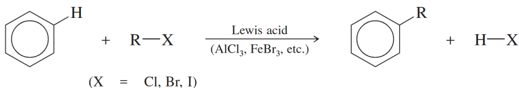
Figure 17.6 Friedel–Crafts alkylation
