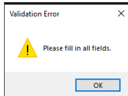
Figure 4. Validation Error
