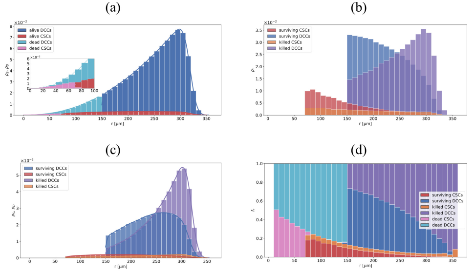
Fig 5. Combined effects of hypoxia and radiation on 30-day tumorspheres. (a) Cell distribution before the therapy. The spheroid has developed a necrotic core of radius R_N = 150 \mu\text{m} . The inset highlights the hypoxic CSC range. (b) Cell distribution after a single dose of radiotherapy; the fraction of killed DCCs in the necrotic core is greater than that of killed CSCs. (c) Histograms from (b) rescaled to show the radial dependence of the cell concentration. (d) Concentration fractions of all cell types. Here c_S = 0.23 and c_D = 0.30 .
