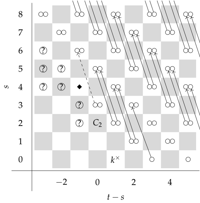
Figure 1.1: E_3 -page of the limit spectral sequence for computing the Picard group of \text{StMod}(kQ_8) . The nontrivial differentials have been illustrated.
