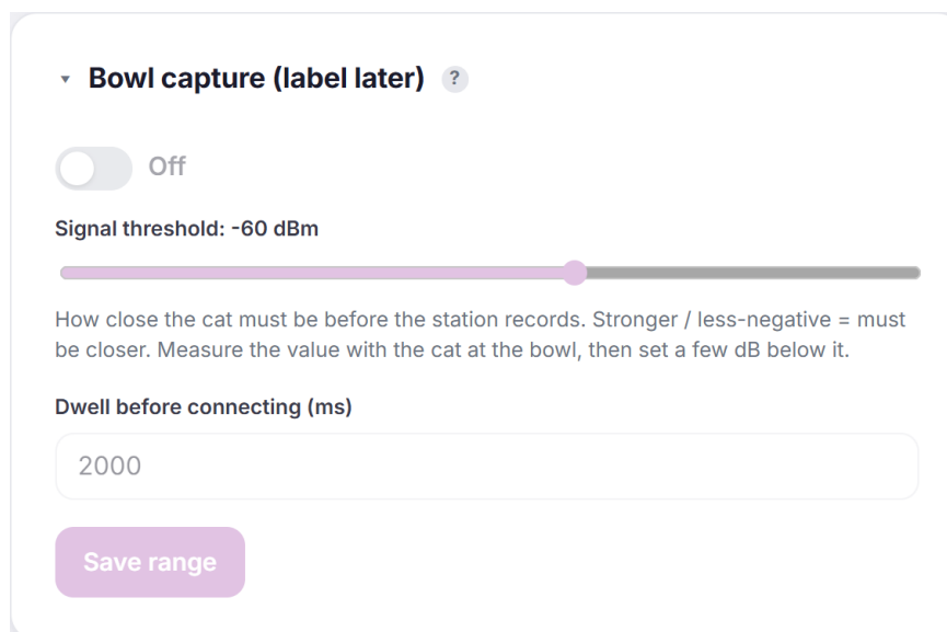
Figure 22: Bowl capture: the range gate (signal threshold and dwell) for unattended recording.
