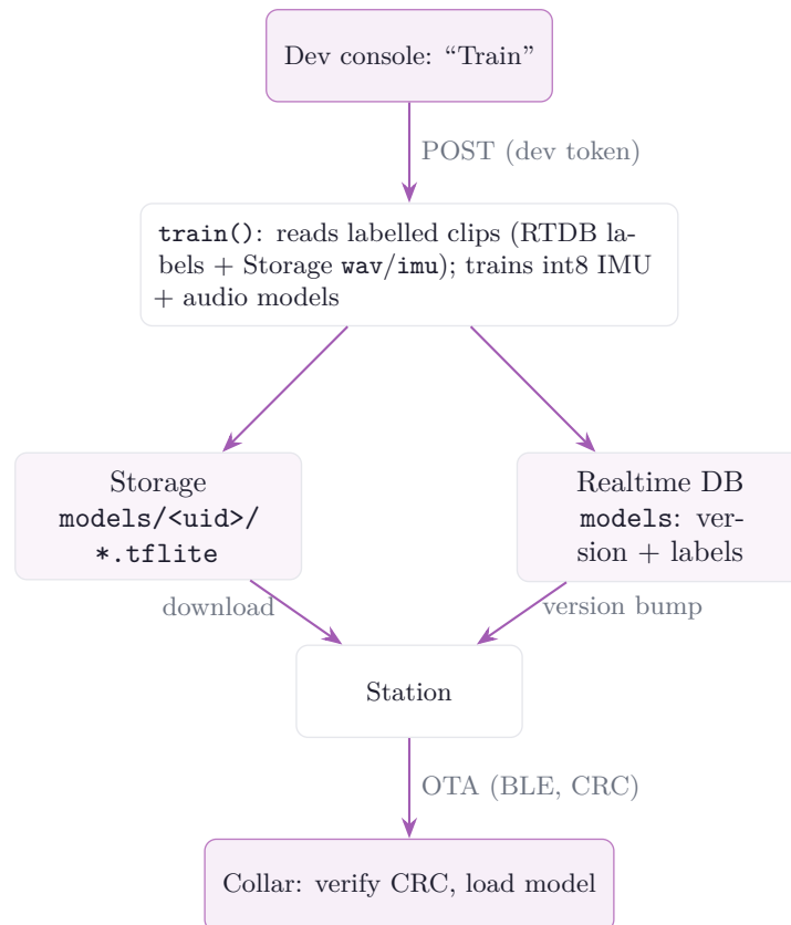
Figure 6: Training and over-the-air model delivery. train() reads the labelled clips, writes the quantised models to Storage and the new version and labels to the database, and the station detects the version bump, downloads the models, and pushes them to the collar.
